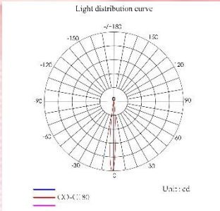
Light Distribution chart
